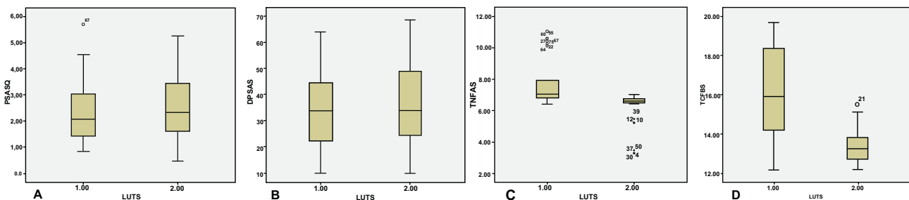
Fig. (1). Levels Differences in case and control groups: 1A: PSA ( p=0.452 ); 1B: PSA density ( p=0.754 ); 1C: TNF- \alpha ( p=0.00 ); 1D: TGF- \beta ( p=0.000 ).
