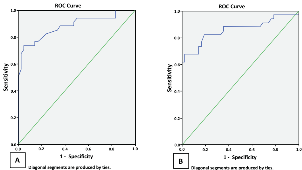
Fig. (2). ROC Curve of TNF- \alpha (2A) and TGF- \beta (2B).
